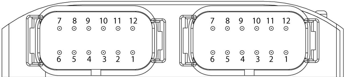
Key DTM04-12PA
